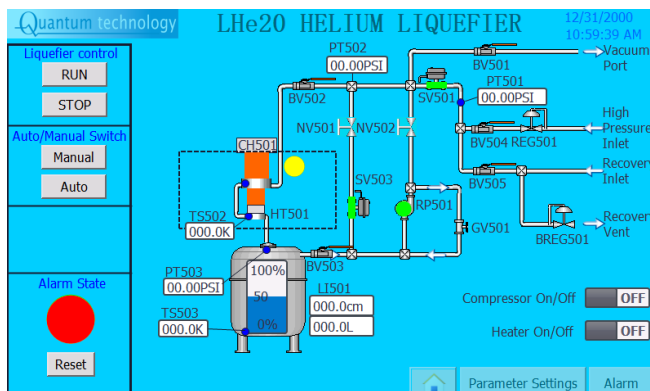
Quantum mobile liquefier HMI,
